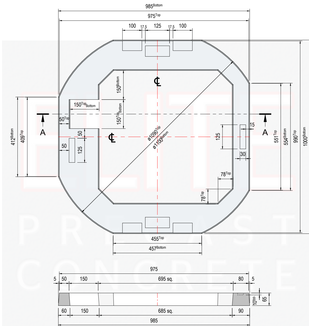
Section Thro Arrow A - A
