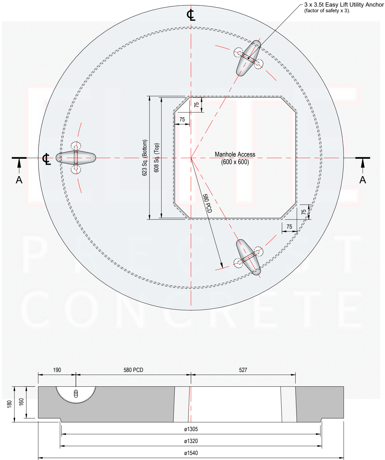
Section on Arrow A - A
