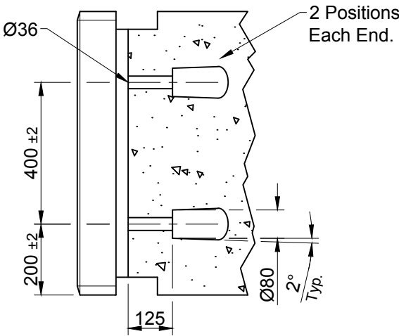
Part Section Arrow A - A Detail Identical Both Ends
