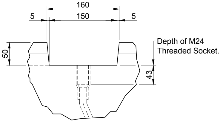
Channel Detail Scale 1:5
