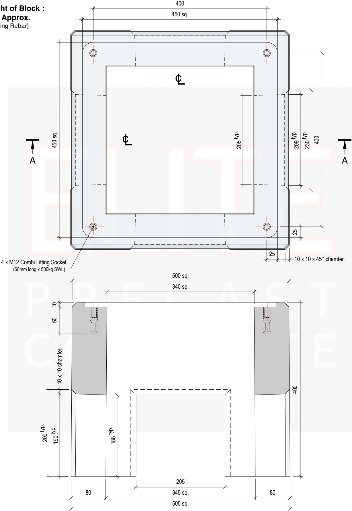
Section on Arrow A - A
