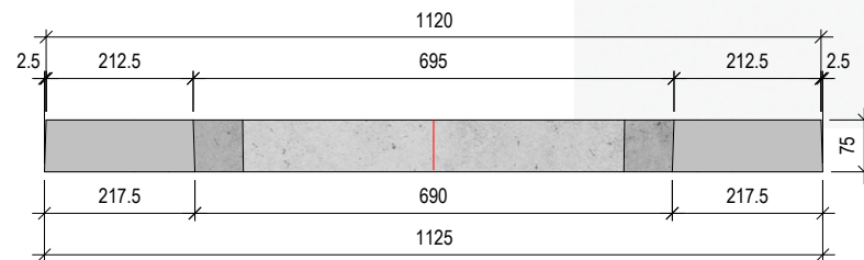
Section on Cut Line A - A
