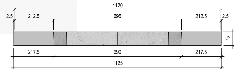
Section on Cut Line B - B
