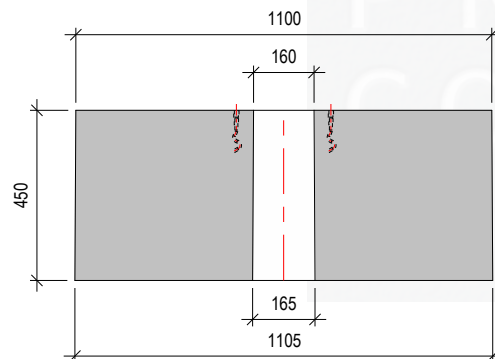
Section on Cut Line A - A
