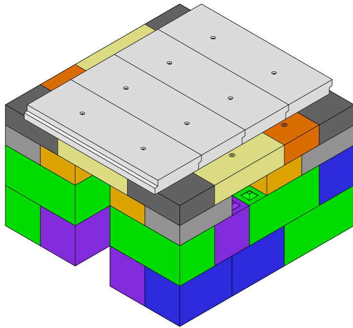
Option A - Standard Silo Cover Slab Roof
