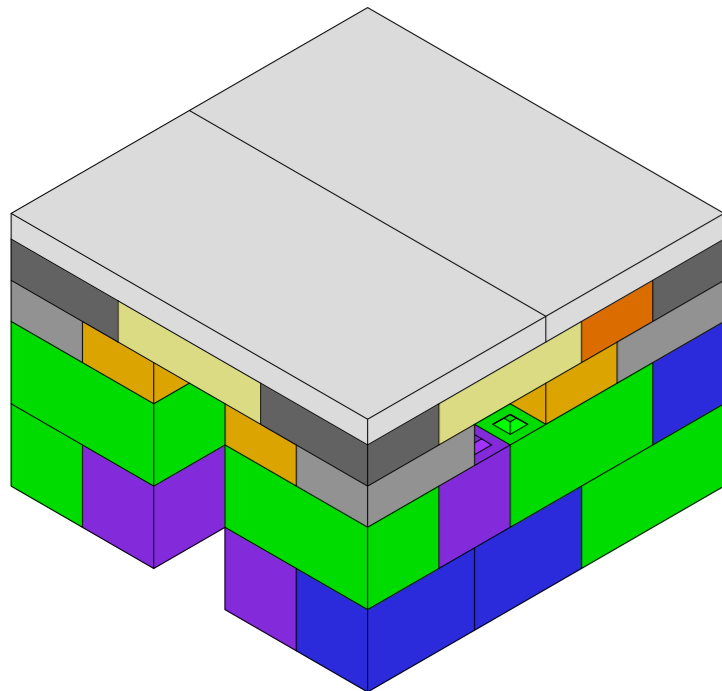
Option B - Specialised Roof Slabs
